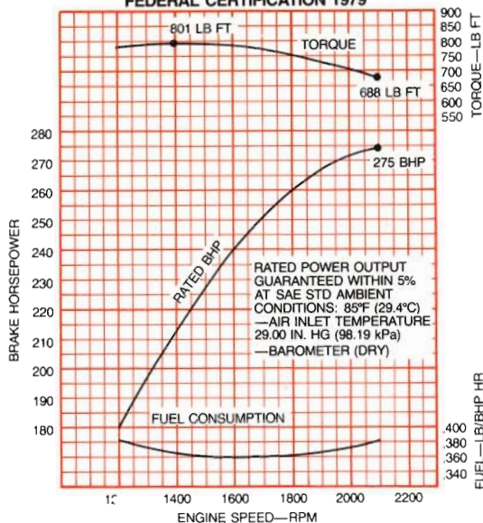
BASIC ENGINE PERFORMANCE MODEL 6-71T WITH 7C75 INJECTORS FEDERAL CERTIFICATION 1979
