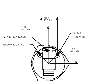
ENLARGED VIEW OF CHARGING GENERATOR
