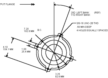
EXHAUST OUTLET-ENLARGED VIEW 2 PLACES
