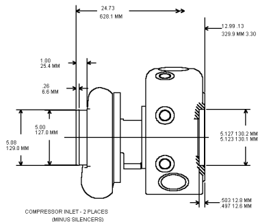
COMPRESSOR INLET - 2 PLACES (MINUS SILENCERS)
