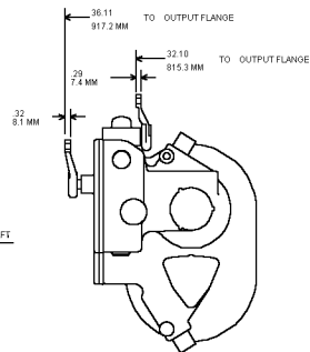
VARIABLE SPEED GOVERNOR ENLARGED VIEW
