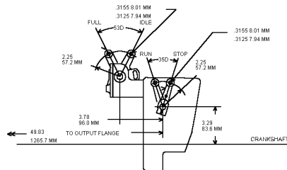
VARIABLE SPEED GOVERNOR ENLARGED VIEW
