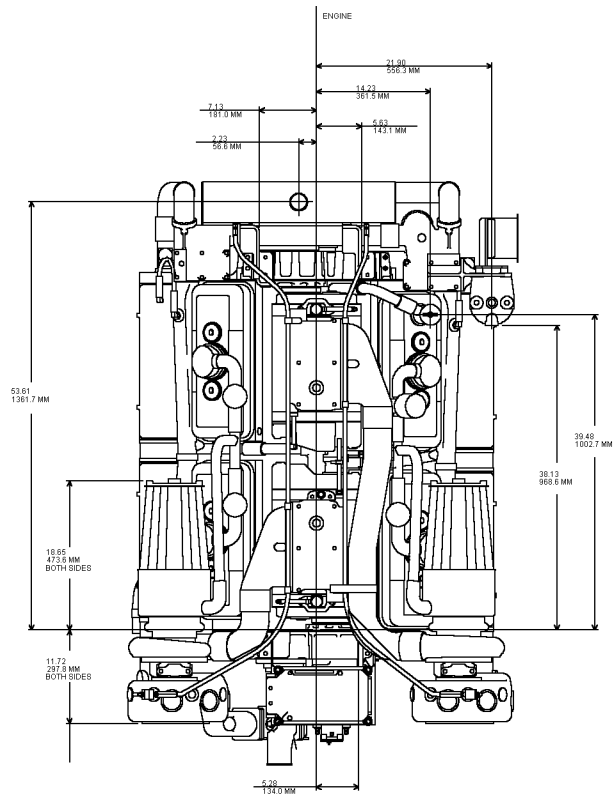
TOP VIEW
