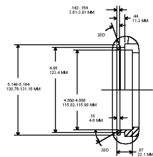
TURBO EXHAUST OUTLET ENLARGED VIEW
